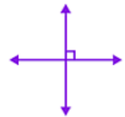
Perpendicular lines
